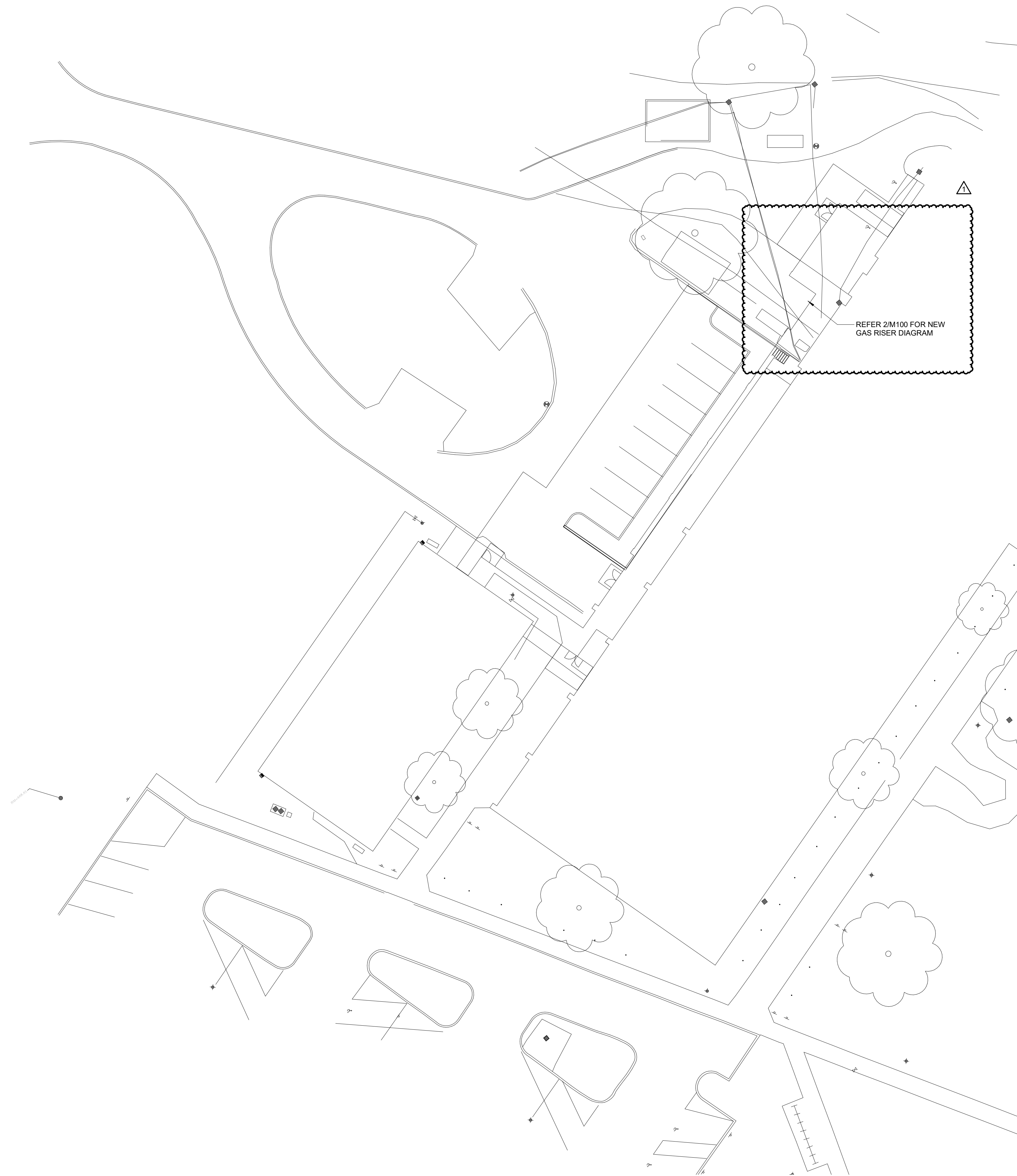
1 SITE - MECHANICAL 1" = 20'-0"
